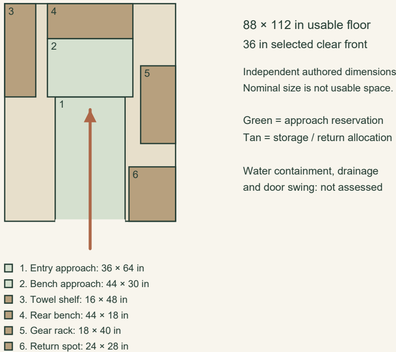
ShedBuildPlans · Original diagram · Not to construction scale
